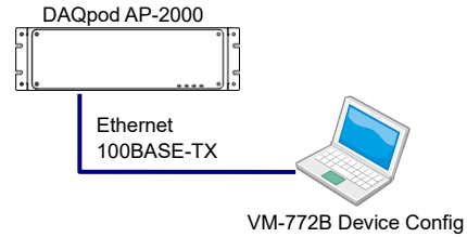
Connecting to DAQpod AP-2000 infiSYS Data Acquisition Unit (Connecting to Ethernet port)
