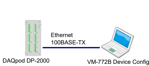
Connecting to DAQpod DP-2000 infiSYS Data Acquisition Unit (Connecting to Ethernet port)
